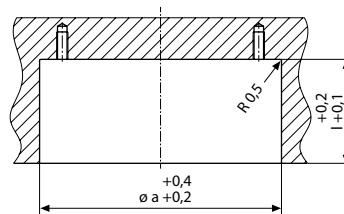
Location hole
